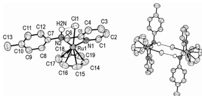
Figure 8. Left: Crystal structure of S_{Ru,\lambda,R_N} - 4a . Right: Assembly of pairs of enantiomers R_{Ru,\delta,S_N} and S_{Ru,\lambda,R_N} . Hydrogen atoms have been omitted for clarity (hydrogen atoms involved in hydrogen bonding interactions are shown). Selected bond distances (Å) and angles (deg): Ru1–C11, 2.403(14); Ru1–N1, 2.093(5); Ru1–N2, 2.139(4); Ru1–C14, 2.182(6); Ru1–C15, 2.166(6); Ru1–C16, 2.159(6); Ru1–C17, 2.175(7); Ru1–C18, 2.192(6); Ru1–C19, 2.168(6); N1–Ru1–C11, 84.83(12); N2–Ru1–C11, 83.34(13); N1–Ru1–N2, 76.86(16).
