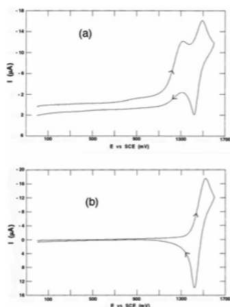
Figure 9. Cyclic voltammograms of 2a (a) and 8a (b). In dichloromethane, 0.1 M [NBu_4]^+ [PF_6]^- at a Pt bead electrode. Scan rate = 100 mV s -1 .
