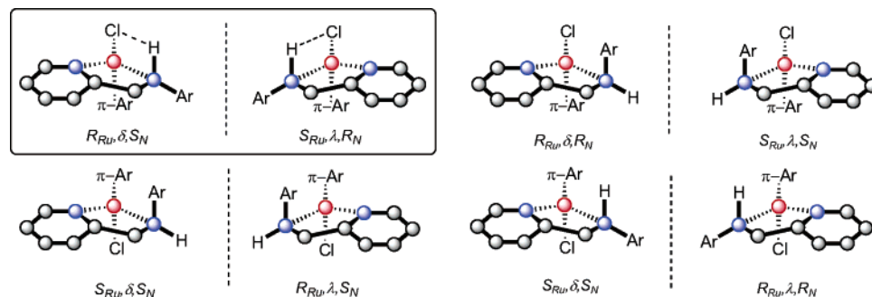
Figure 7. Eight possible geometric isomers for cationic complexes 4^+ and 5^+ . Only the framed couple of enantiomers R_{Ru}, \delta, S_N and S_{Ru}, \lambda, R_N is actually formed.
